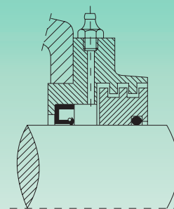
Obtención de taconite "TAC" para: SN-SD "TAC" taconite cover for: SN-SD
